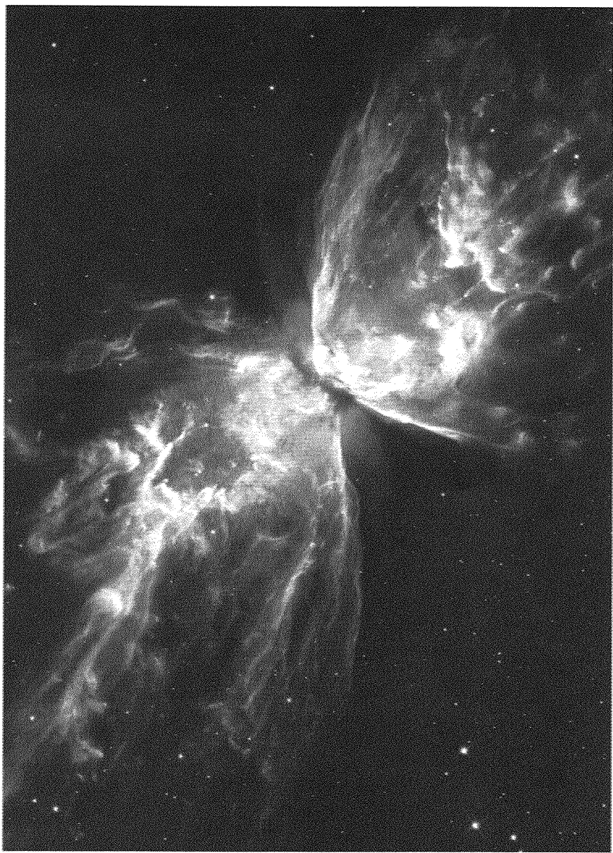
The Butterfly Nebula, discovered in 1947 by astronomer Rudolph Minkowski, has the peculiar form of two lobes that emanate from a central star, resembling the wings of a butterfly. This image was captured by the Hubble Space Telescope in 2009.
